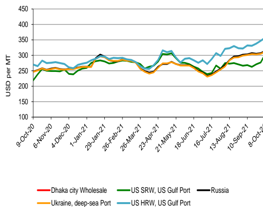
Figure 4: Wheat wholesale price in Dhaka and FOB Prices in relevant international markets
